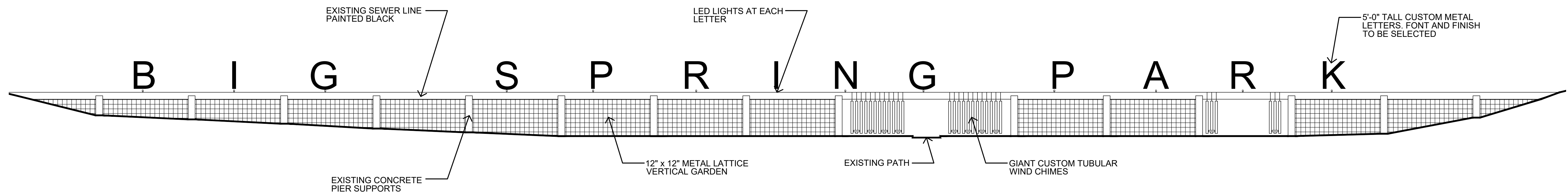
4 Pipeline Improvement - Elevation - Concept B 3/32" = 1'-0"
